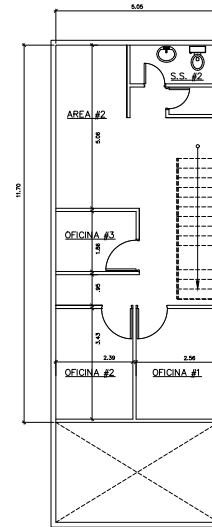
MEZZANINE ESC. 1:1100
